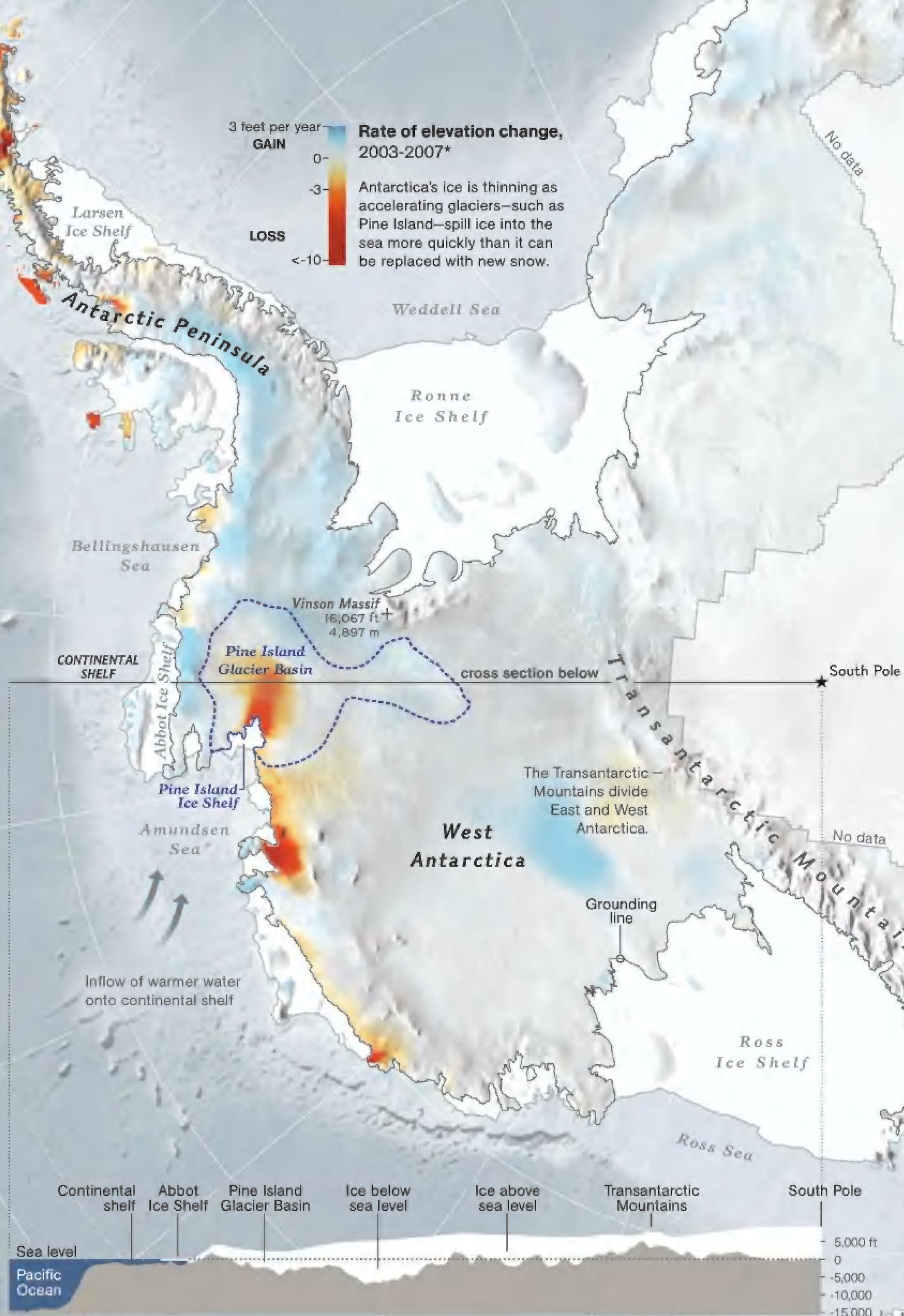
Below the icy surface This cross section shows that in the Amundsen Sea region, much of the ice slides on a bed that's below sea level, where relatively warm, deep water is contributing to the thinning of ice shelves.
